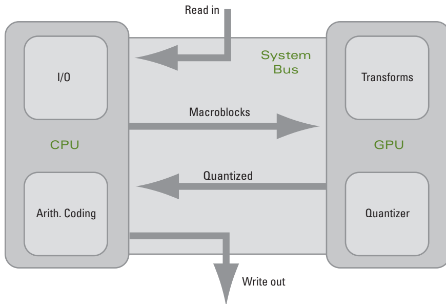
Figure 2 – CPU-GPU architecture.
