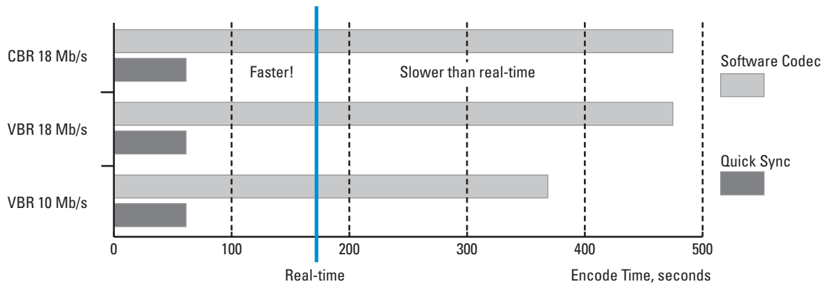
Figure 5 – AVCHD benchmark.
