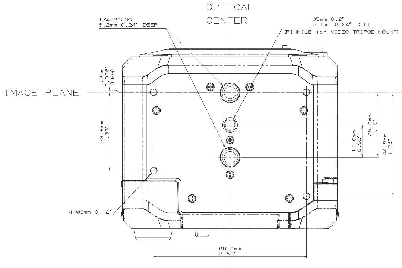
CAMERA BOTTOM
