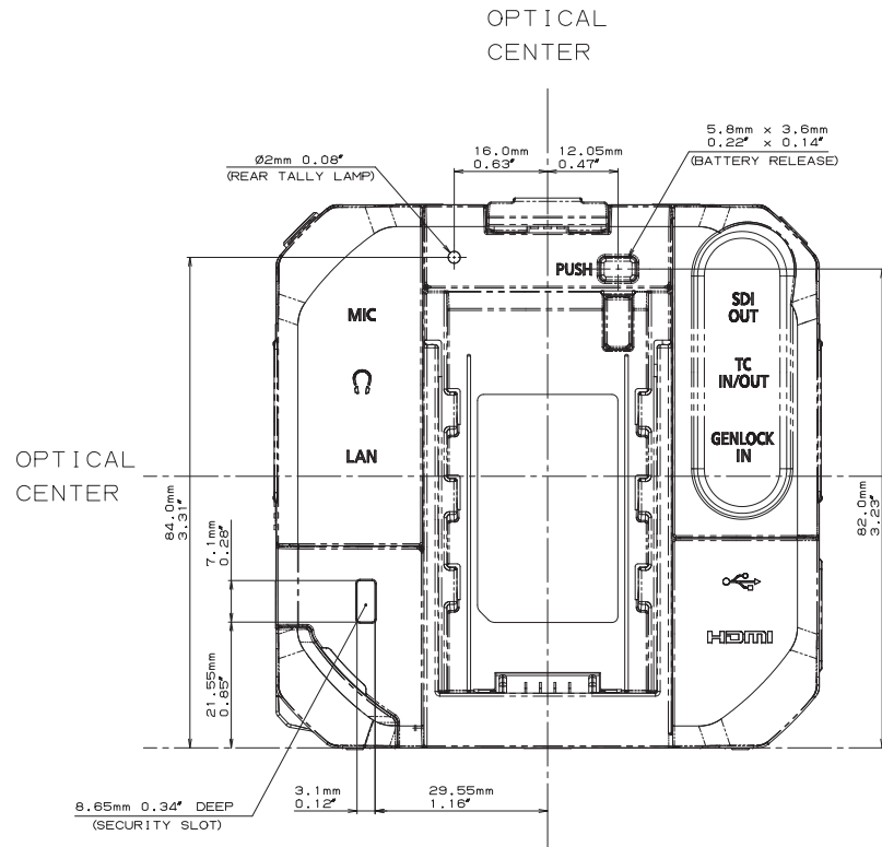
CAMERA BACK
